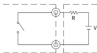
Fig 2.2 Internal circuit of AC OK (Battery Low)
